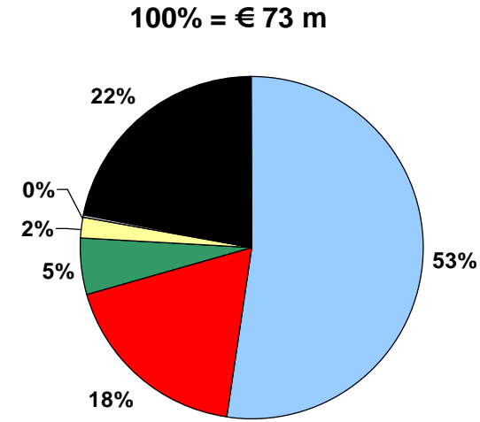
Net Profit
