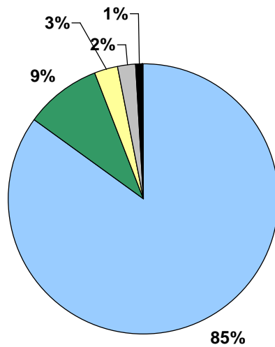
Revenues
