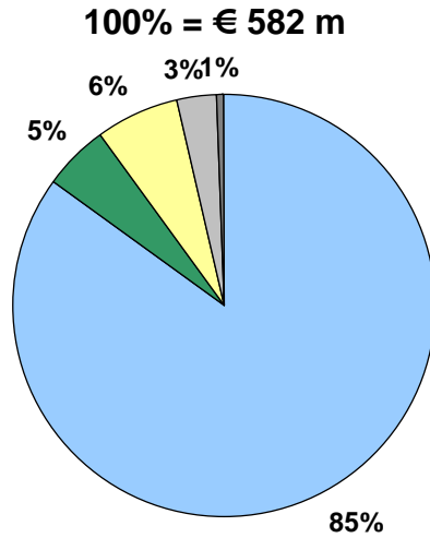
Revenues
